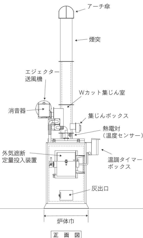
図面はMDP-400M
